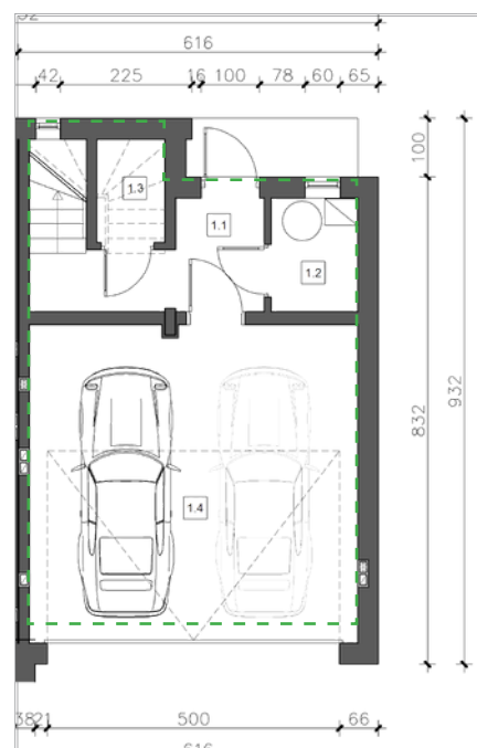
PARTER
