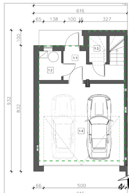
PARTER
